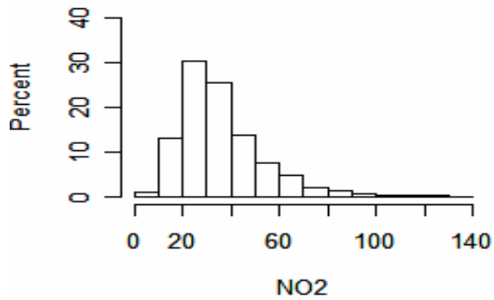
Histogram of NO2
